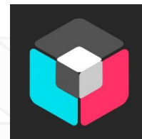
School app
